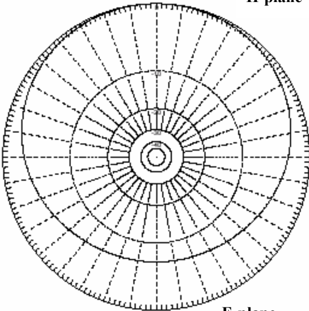
E-plane Gain 6,26dB
